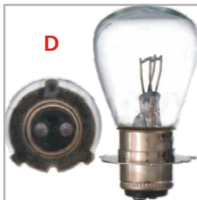
P15D-3 Dual Contact (J Type)
