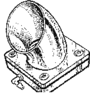
585-9491 Flange Size 2" O.D. Venturi Diameter: 1.845" ID # of mtg bolts: 4 Bolt Circle Diameter: 2.5"
