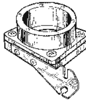
585-9000 Carburetor Bracket use with adapter Part #585-9294 on '94-96 Sea Doo GTX, HX, SPX & XP Prevents intake manifold from cracking Use 1 bracket per vessel
