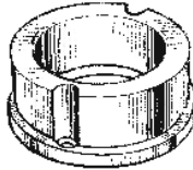
585-9265 Flange Size 2 3/4" O.D. Venturi Diameter: 1.645" I.D. # of mtg bolts: 2 Bolt Circle Diameter: 2.65"
