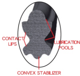
RX RING CUTAWAY
