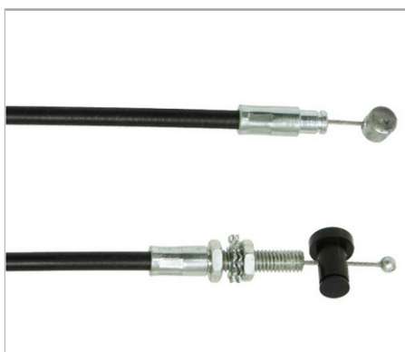
724-38218 Throttle Cable 05-138-209
