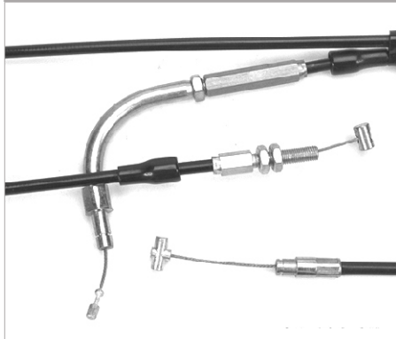
724-3937 Throttle Cable 05-139-37
