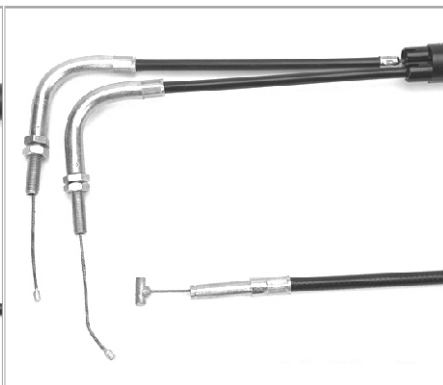
724-3942 Dual Throttle 05-139-42
