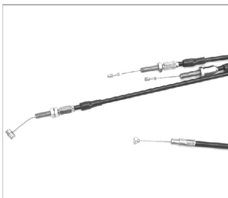
724-3961 Dual Throttle 05-139-61
