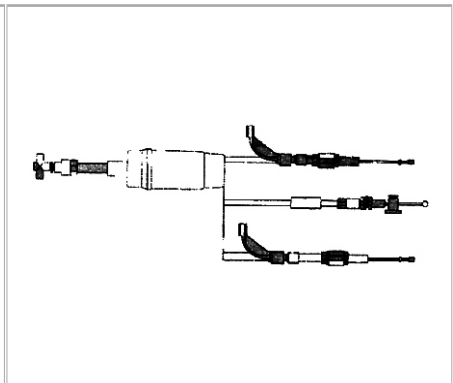
724-4019 Throttle Cable 05-140-19
