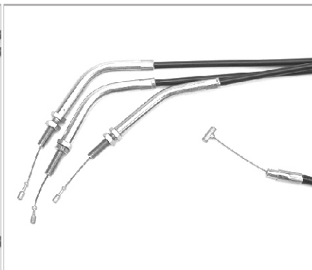
724-3950 Triple Throttle 05-139-50
