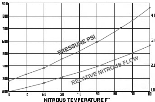
NITROUS OXIDE PRESSURE AND FLOW RATE VS. TEMPERATURE
