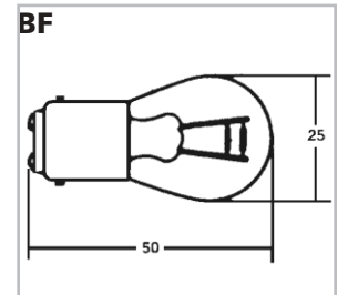
BA15D
