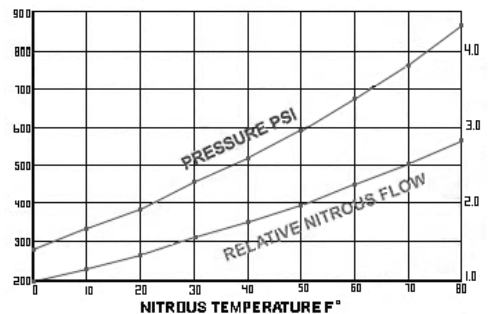
NITROUS OXIDE PRESSURE AND FLOW RATE VS. TEMPERATURE
